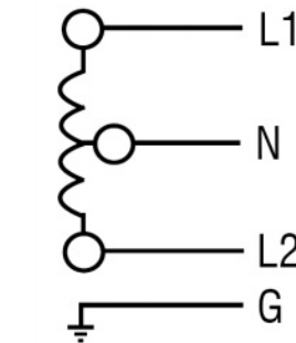
Split Phase 3 Wire + Ground
